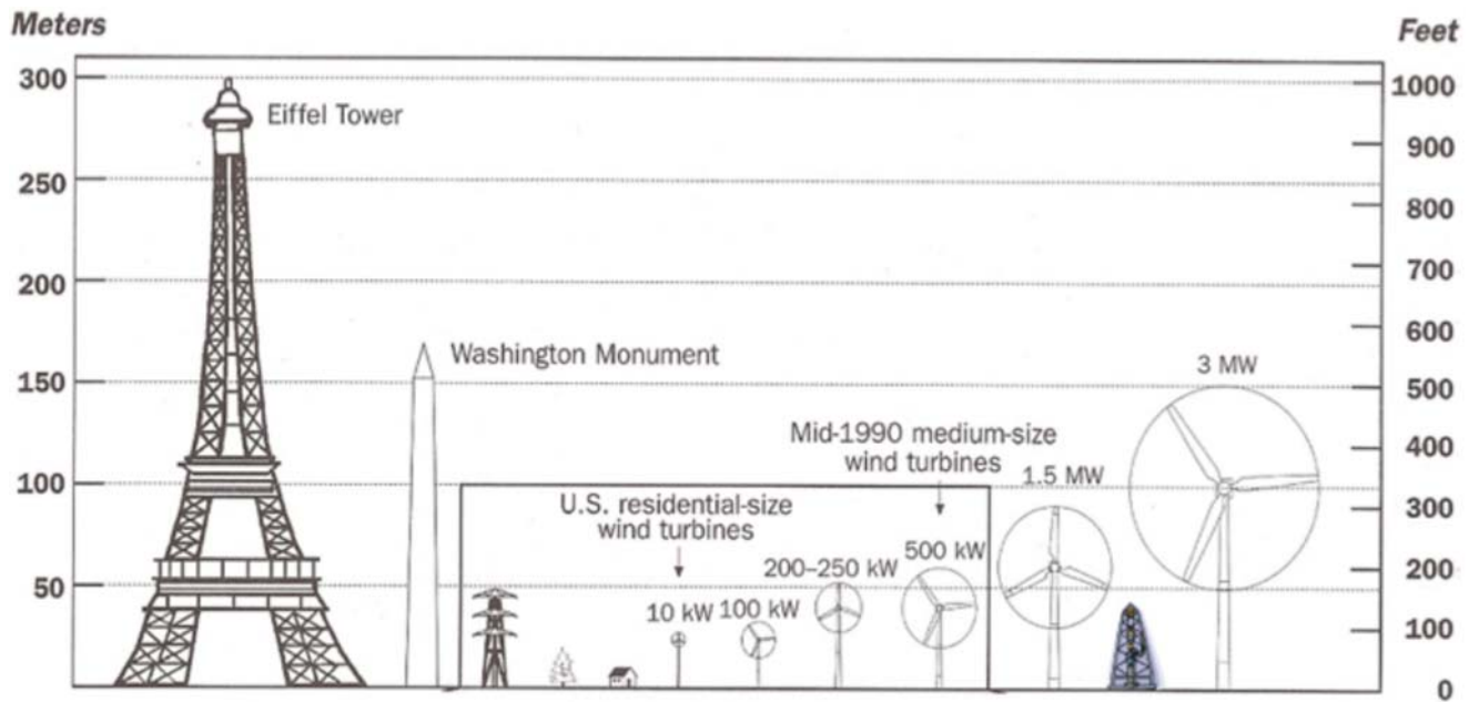
Figure 18. Turbine Scales.
