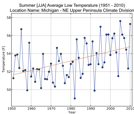
Figure 6. Region-wide temperature trends across Northeast Upper Peninsula of Michigan from 1951 to 2010 for summer daily maximum temperature (right), summer daily minimum temperature (below left), winter daily maximum temperature (below center), and winter daily minimum temperature (below right)
