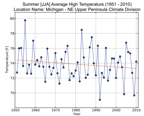
Figure 6. Region-wide temperature trends across Northeast Upper Peninsula of Michigan from 1951 to 2010 for summer daily maximum temperature (right), summer daily minimum temperature (below left), winter daily maximum temperature (below center), and winter daily minimum temperature (below right)
