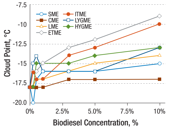
Figure 7. Biodiesel/Diesel Blend Cloud Point Test Results (0%–10% Biodiesel Blend Range)
